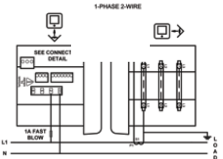
1-phase 2-wire
