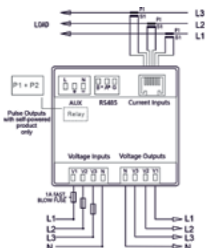
3-phase 4-wire
