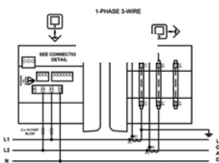
1-phase 3-wire
