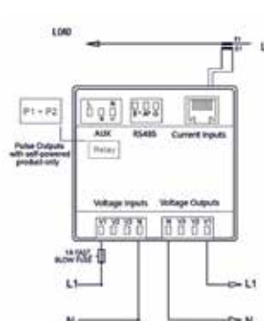
1-phase 2-wire
