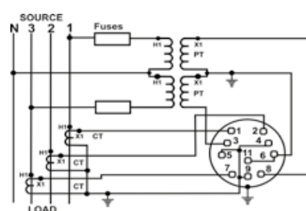
Fig. A3 Models 007-219, 078-219 Wattmeter 3-phase 4-wire unbalanced load
