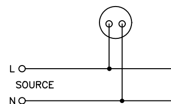
Frequency meter
